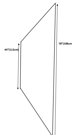
Shawl Schematic
